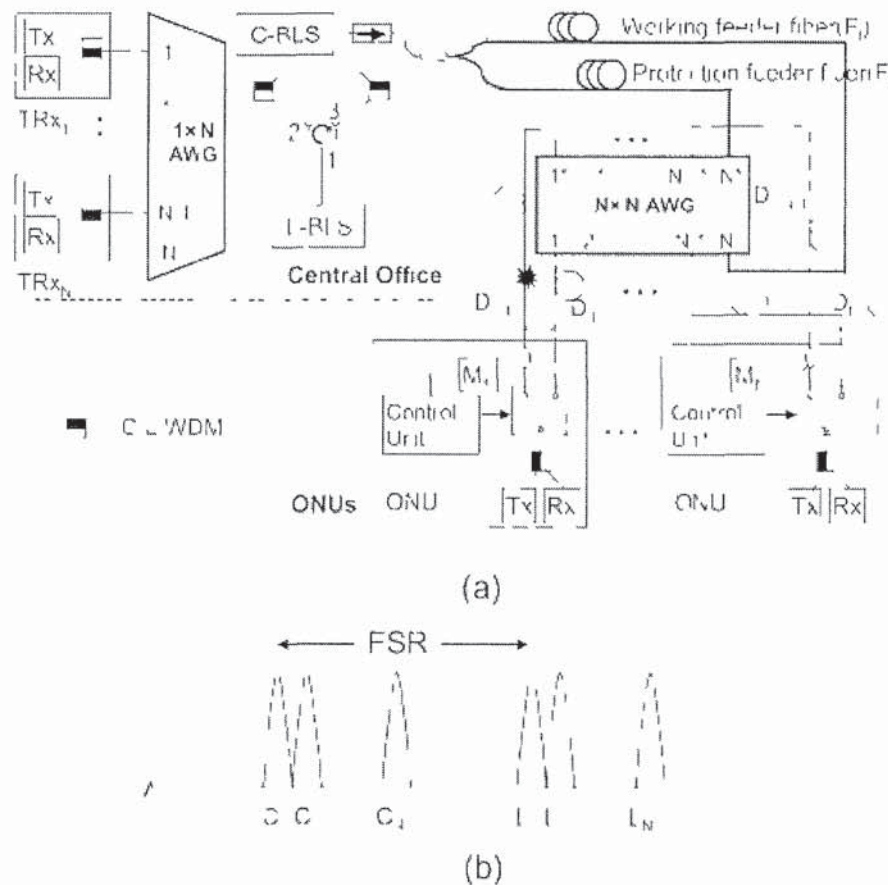
Fig. 4.5 Another protection architecture for WDM-PONs and its wavelength assignment plan in [70]
