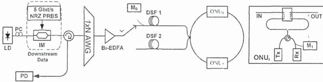
Fig. 4.19 Experimental setup for the proposed WDM/TDM hybrid PON with two ONUs.
