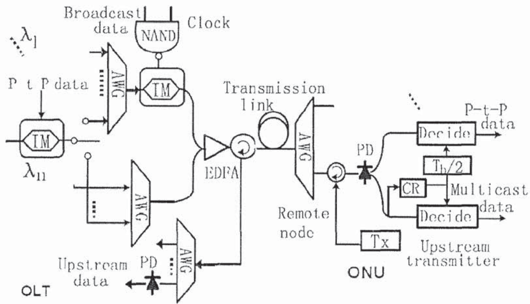
Fig. 3.6 Another multicast enabled WDM-PON architecture employing IRZ [62]
