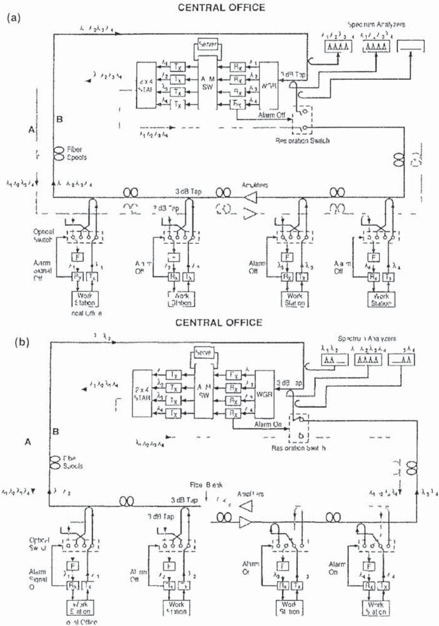
Fig 4.7 A restorable WDM ring network in [72] (a) Schematic of the network under normal condition (b) Schematic of the network with a fiber break
