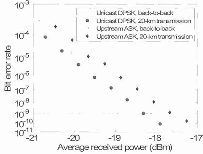
Fig. 3.26 BER measurements when multicast is disabled
