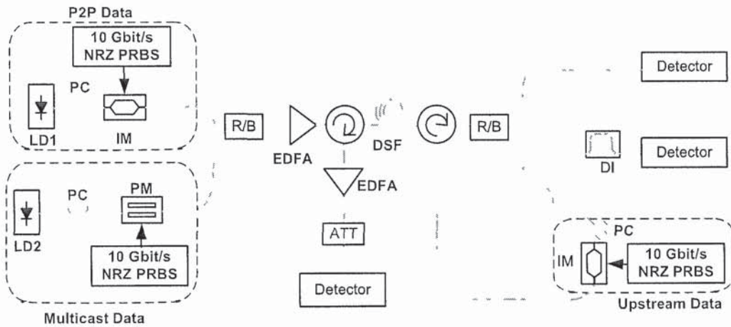
Fig. 3.9 Experimental setup of proposed polarization-assisted WDM-PON. IM: optical intensity modulator, PM: optical phase modulator, DI: delay interferometer, PC: polarization controller, R/B: Red/blue filter, ATT: optical attenuator, EDFA: Erbium-doped fiber amplifier, DSF: dispersion-shifted fiber.
