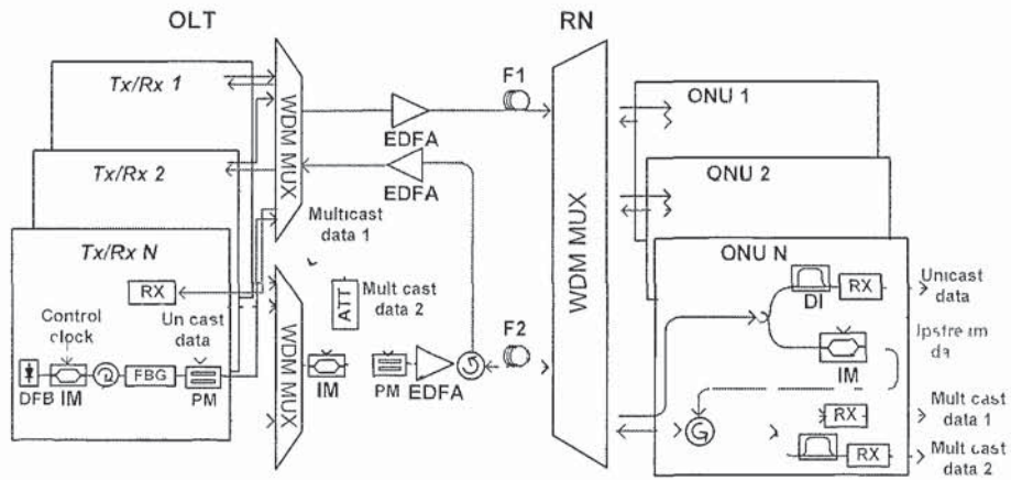
Fig. 3.29 A WDM-PON with an overlay scheme to realize simultaneous transmission of two sets of multicast data. F1 & F2: fiber feeders, FBG: fiber Bragg grating, IM: optical intensity modulator, EDFA: Erbium doped fiber amplifier, DI: delay interferometer.
