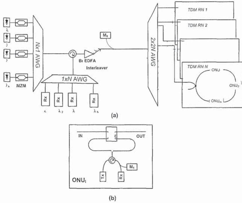
Fig 4 17 Proposed survivable architecture for WDM/TDM PONs (a) Configuration of the proposed network (b) Schematic diagram of the ONU module M_{0/1} monitoring unit
