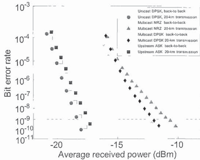
Fig. 3.31 BER measurements when two multicasts are enabled.
