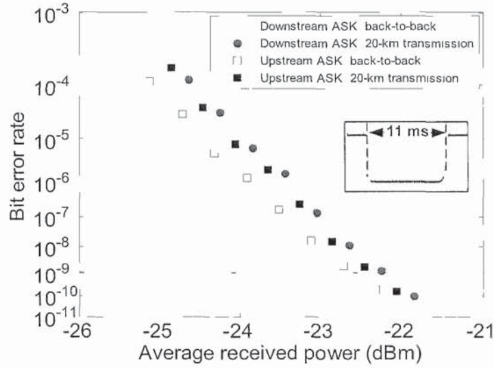
Fig. 4.21 BER measurements for ONU_2 in case of a fiber cut between ONU_1 and ONU_2 .
