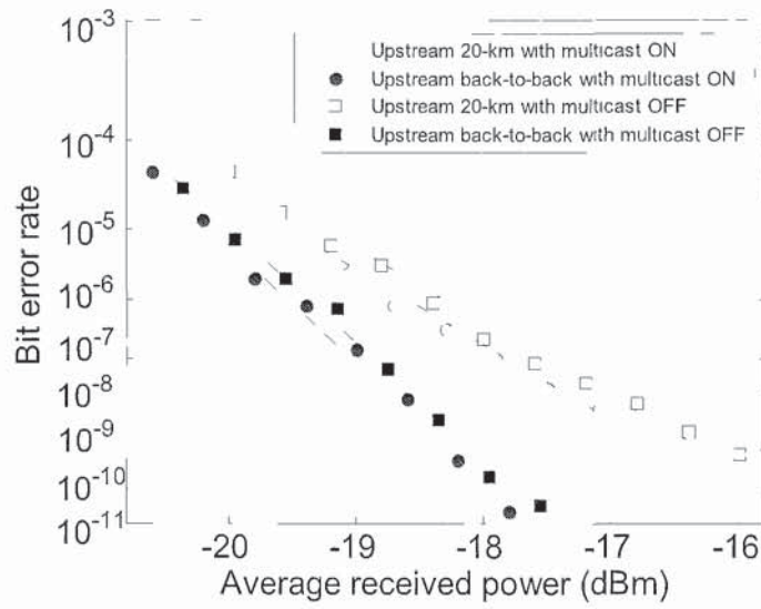
Fig. 3.12 BER measurements of 10-Gb/s upstream transmission Multicast-enabled ( \bullet , \circ ), multicast-disabled ( \blacksquare , \square )
