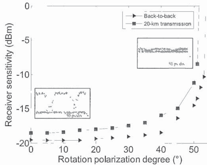
Fig. 3.10 Measured performance of the demodulated DPSK signal versus the input polarization to the optical phase modulator. Insets show the respective eye diagrams at different input polarizations.
