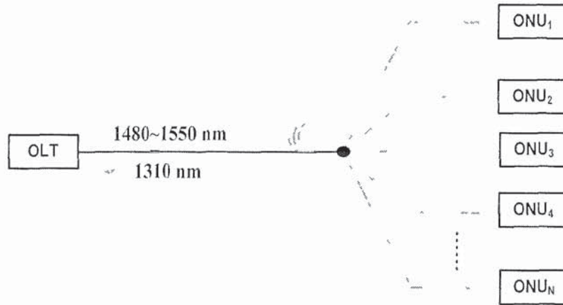
Fig. 1.2 The architecture of a TDM-PON
