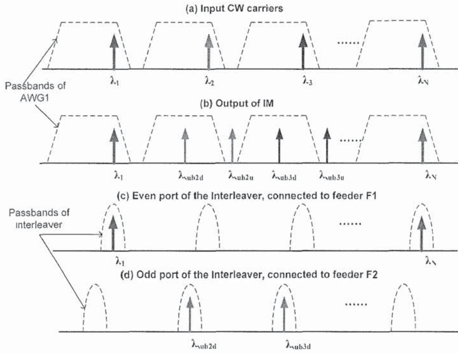
Fig. 4.13 Spectra of downstream carriers to illustrate the protection principle, assuming that fiber failures have been detected along the lightpaths of \lambda_2 and \lambda_3 , for example.
