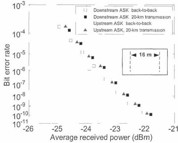
Fig 4 22 BER measurements for ONU_2 when a fiber cut occurs in DSF1
