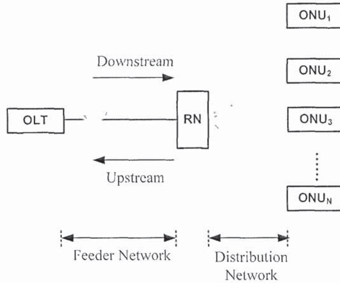
Fig. 1.1 The architecture of a passive optical network
