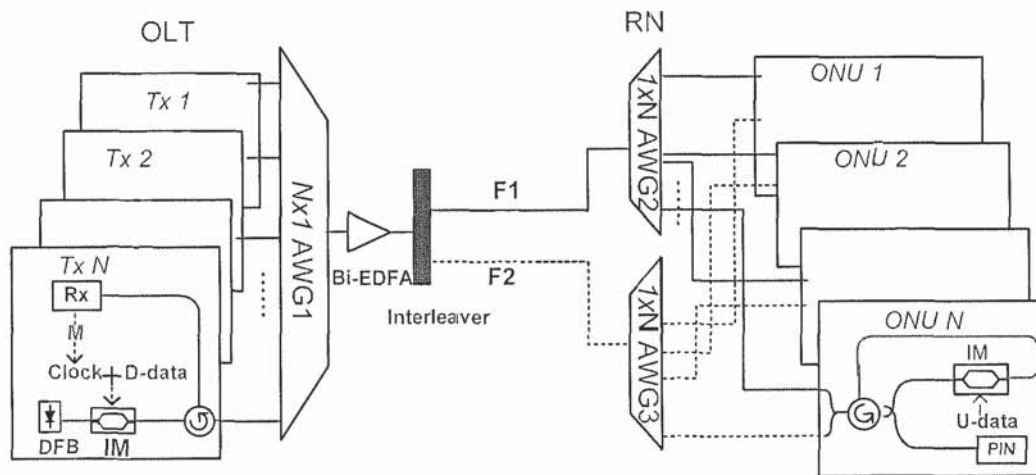
Fig. 4.12 The WDM-PON with proposed self-protection scheme. IL: optical interleaver, M: monitoring unit.
