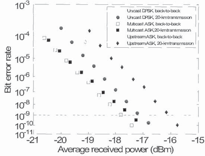
Fig. 3.28 BER measurements with multicast enabled when the control clock frequency is 15-GHz.
