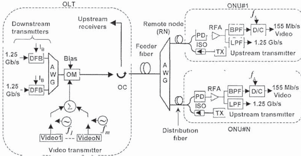
Fig. 3.2 Multicast enabled system utilizing subcarrier multiplexing [58]
