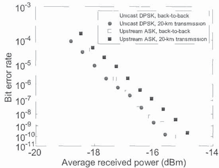
Fig. 3.22 BER measurements when multicast is disabled
