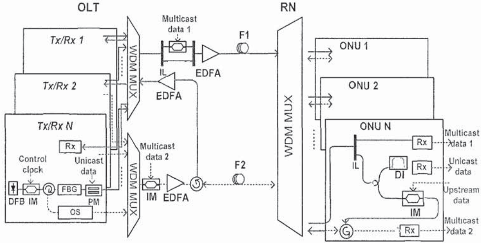
Fig. 3.32 Proposed WDM-PON with multicast overlay supporting two independent multicast streams. IL: optical interleaver; MUX/DEMUX: wavelength multiplexer/demultiplexer; OS: optical on/off switch.
