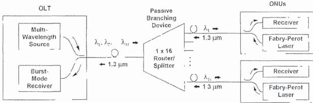
Fig. 2.2 Schematic of a single-fiber CPON [23]
