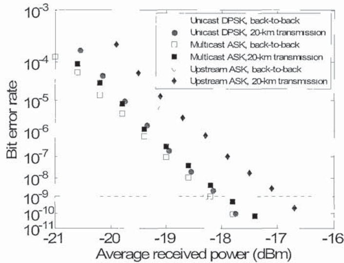
Fig. 3.27 BER measurements with multicast enabled when the control clock frequency is 20-GHz.
