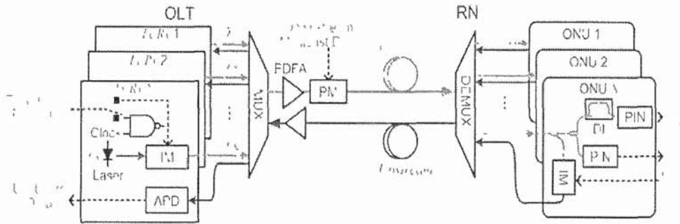
Fig. 3.5 A multicast enabled WDM-PON architecture employing IRZ [61]
