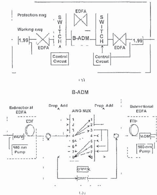
Fig. 4.8 A bidirectional WDM self-healing ring network [73]. (a) Node configuration of the proposed bidirectional self-healing ring network. (b) Schematic diagram of the bidirectional add/drop amplifier module.
