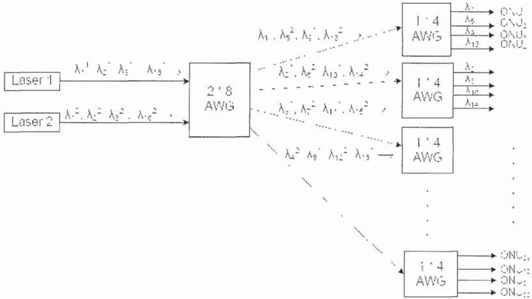
Fig. 2.4 An example of a multistage AWG-based WDM-PON with 32 ONUs [28]
