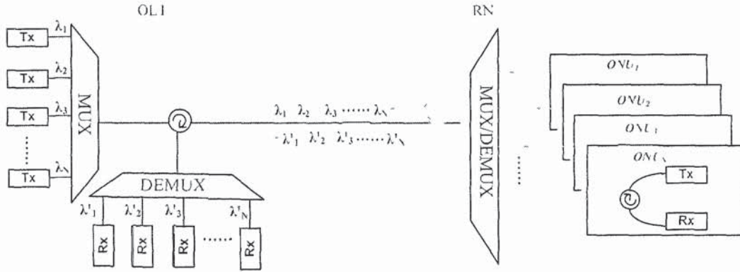
Fig. 1.3 The architecture of a WDM-PON
