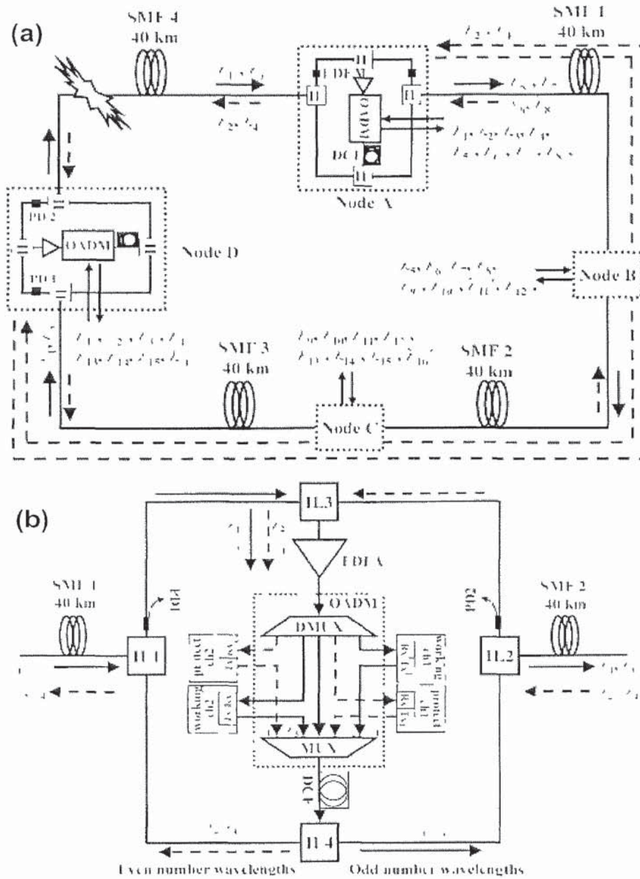
Fig. 4.9 A 1-fiber bidirectional WDM self-healing ring network [74]. (a) Network architecture. (b) Diagram of the optical add/drop multiplexer module (B-OADM).
