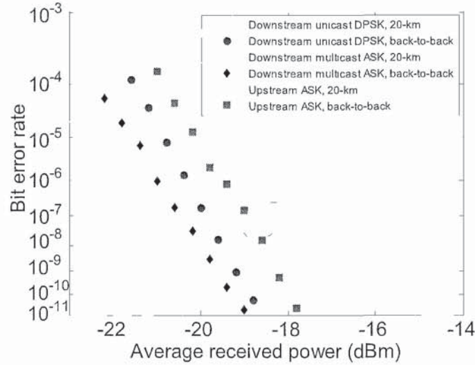
Fig. 3.15 BER measurements of 10-Gb/s transmissions: downstream point-to-point DPSK ( \circ, \bullet ), downstream multicast ASK ( \diamond, \blacklozenge ); upstream ASK ( \square, \blacksquare )
