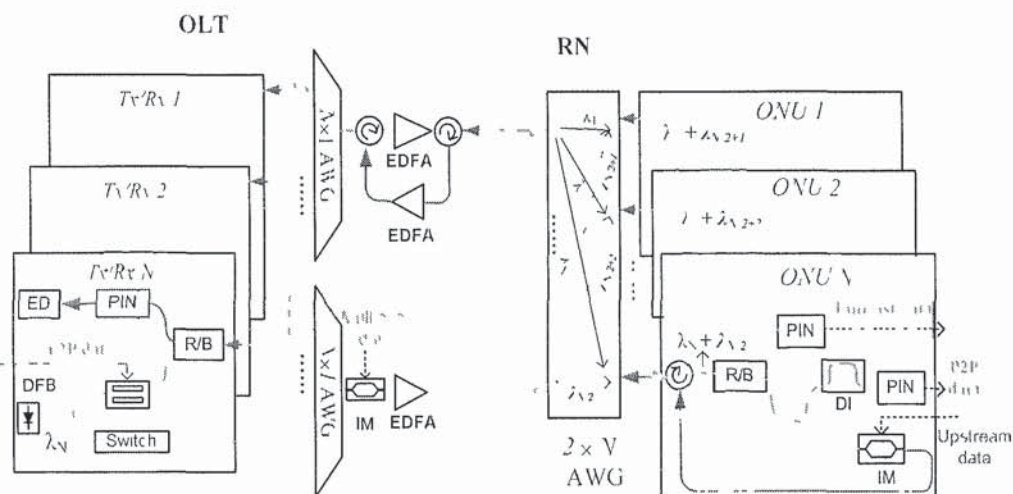
Fig. 3.13 Proposed WDM-PON with switch-assisted multicast overlay control
