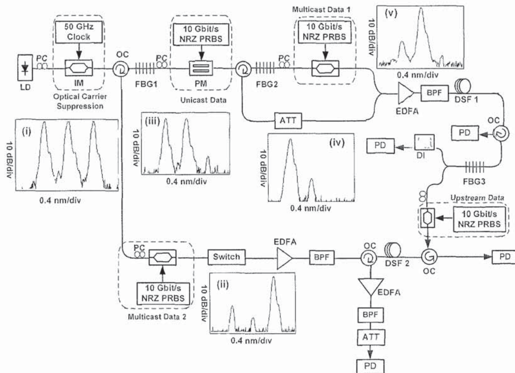
Fig. 3.34 Experimental setup. Insets show the (i) output spectrum of the IM; (ii) reflected spectrum of FBG1 (i.e. Multicast data 2); (iii) transmitted spectrum of FBG1; (iv) spectrum for unicast data; (v) spectrum for Multicast data 1. OC: optical circulator, BPF: bandpass filter, ATT: attenuator.
