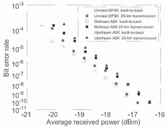
Fig. 3.21 BER measurements when multicast is enabled
