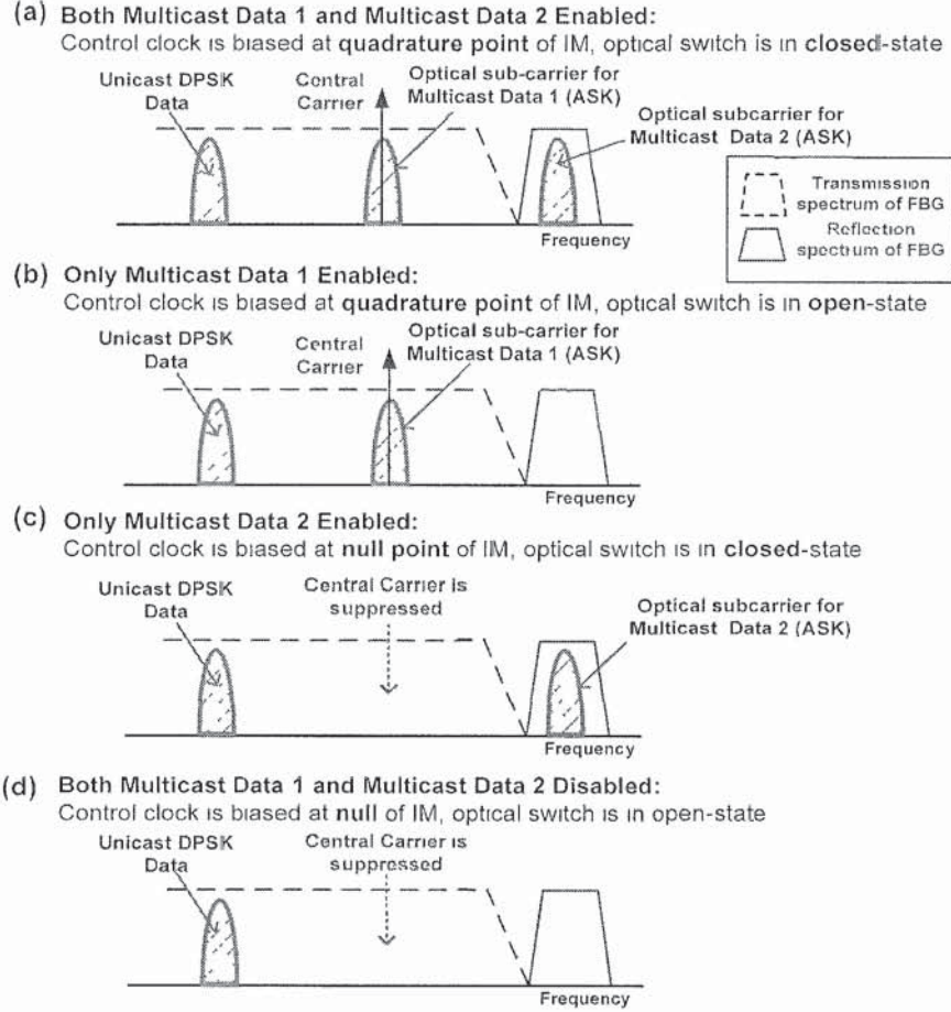
Fig. 3.33 Spectra of downstream carrier to illustrate the principle of multicast overlay fiber control via control clock and optical switch.
