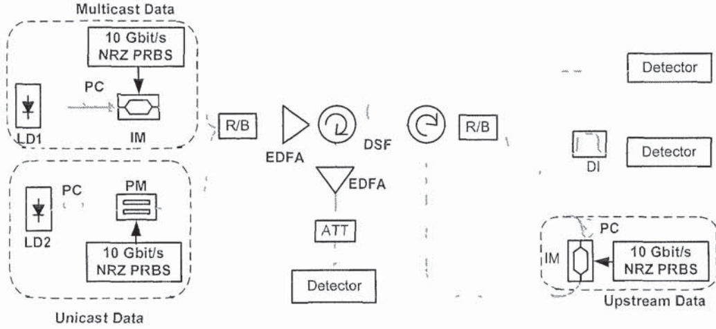
Fig. 3.14 Experimental setup of proposed switch-assisted WDM-PON
