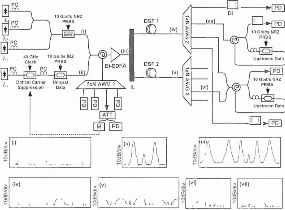
Fig. 4.14 Experimental setup. DSF: dispersion shifted fiber; Bi-EDFA: bi-directional erbium doped fiber amplifier. Insets show the spectra when channel 3 is in its protection mode. Horizontal scale: 0.4nm/div.
