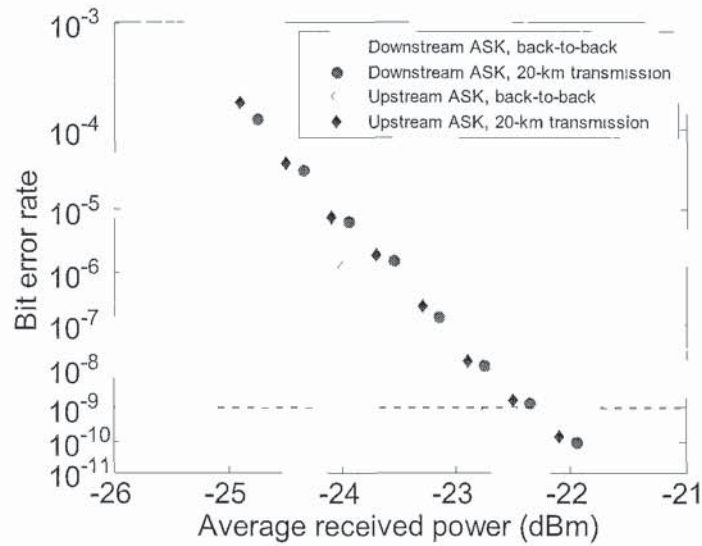
Fig. 4.20 BER measurements for ONU_2 in the normal working mode
