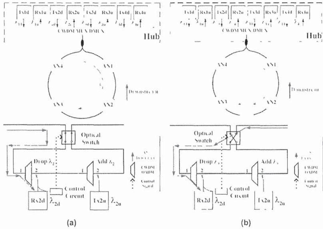
Fig. 4.10 A single-fiber survivable WDM ring network and the structure of the access node (AN) [76]. (a) Under normal mode. (b) Under protection mode.
