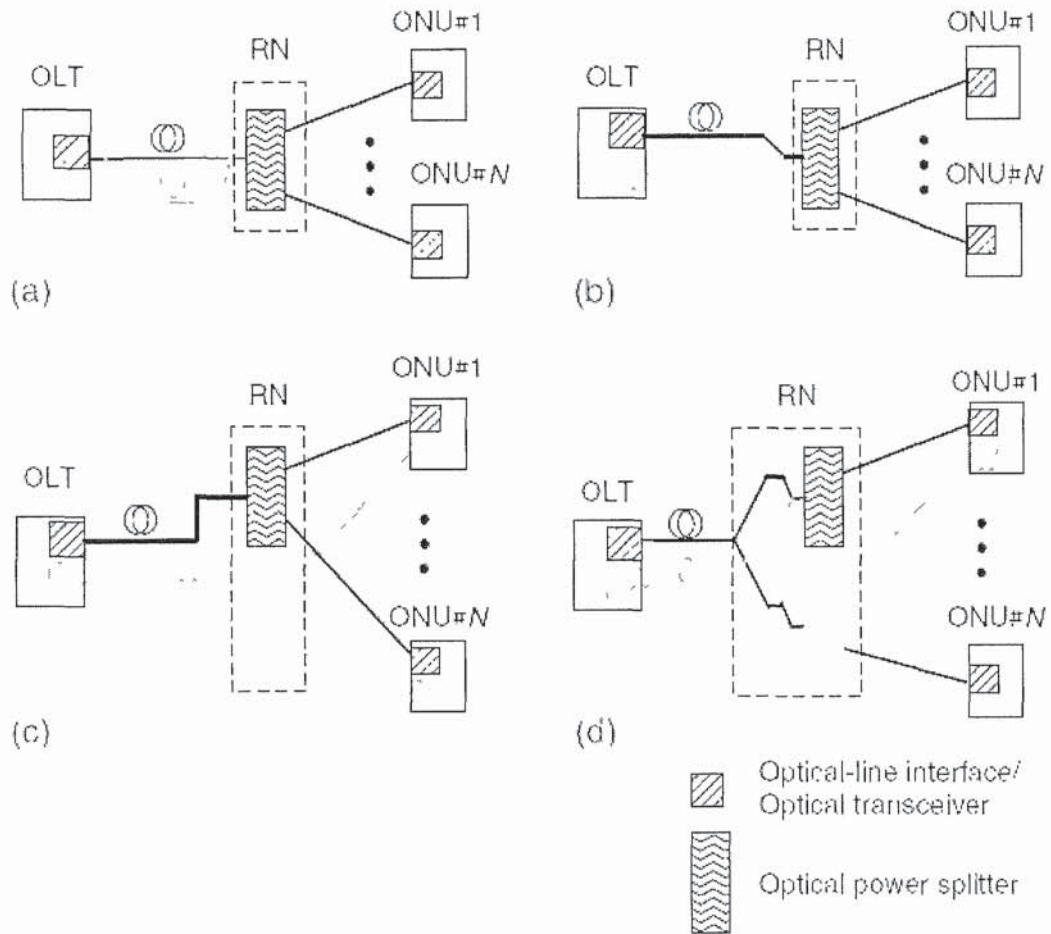
Fig. 4.1 Survivable architectures for PONs suggested by ITU-T G.983.1 [5]
