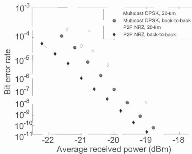
Fig. 3.11 BER measurements of 10-Gb/s downstream transmissions P2P NRZ data:
