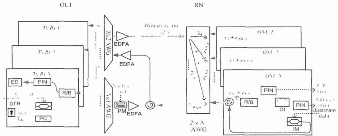
Fig. 3.8 Proposed WDM-PON with polarization-assisted multicast overlay control
