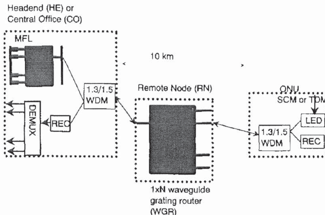
Fig. 2.3 Schematic of architecture of LARNET with N wavelength channels [25]
