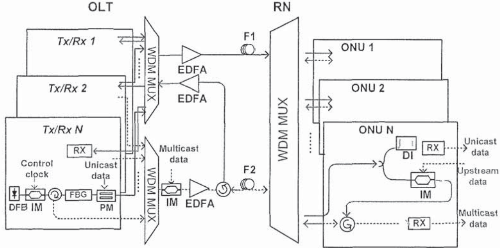
Fig. 3.23 The WDM-PON with modified multicast overlay scheme. F1 & F2: fiber feeders, FBG: fiber Bragg grating, IM: optical intensity modulator, EDFA: Erbium doped fiber amplifier, DI: delay interferometer.
