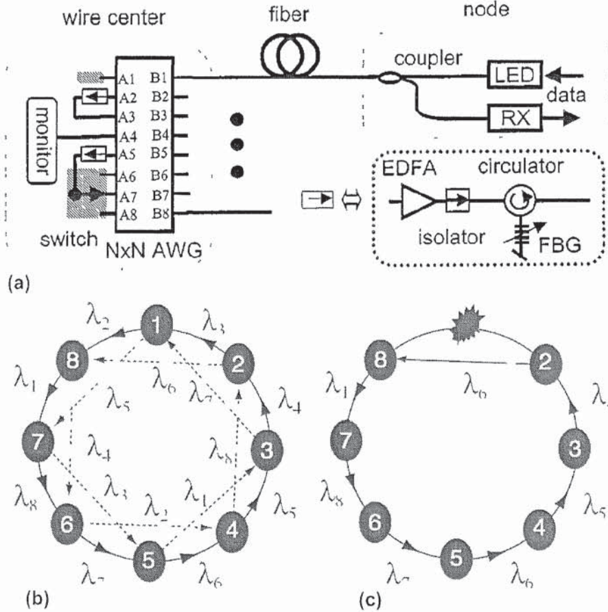
Fig. 4.11 (a) A survivable optical star-shaped ring network; (b) lightpath diagram, dotted lines are the designated protection paths; (c) the protection lightpath is adopted when node 1 failed [78].
