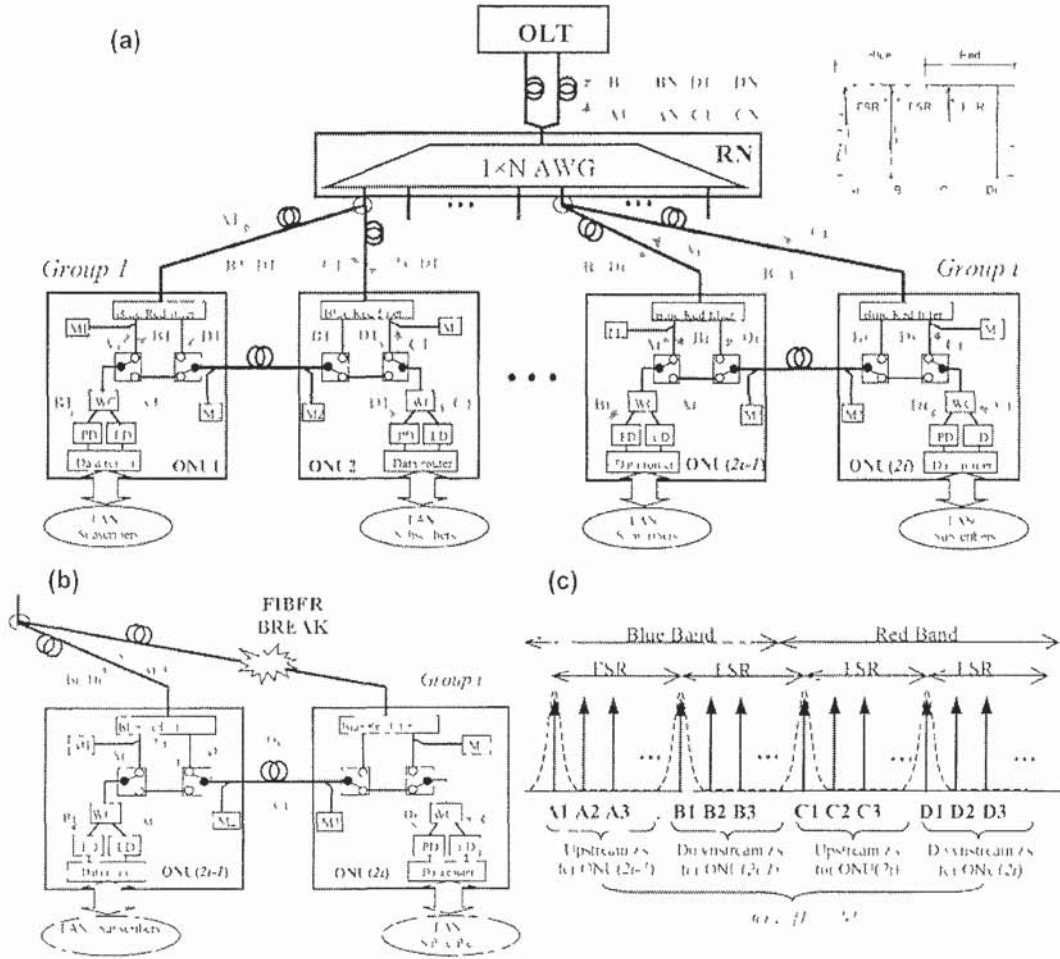
Fig. 4.2 A survivable architecture for WDM-PONs using group protection at the ONU and its wavelength assignment [64]
