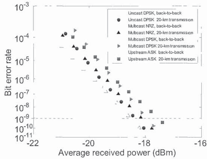
Fig. 3.30 BER measurements when single multicast is enabled.
