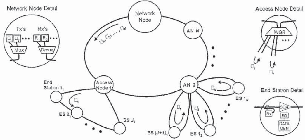
Fig. 2.5 The architecture of a WDM network featuring shared virtual rings [29]
