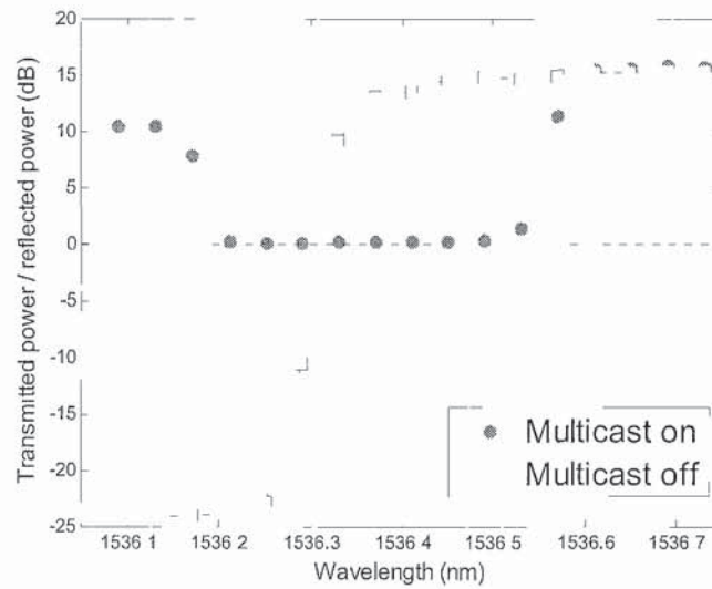
Fig. 3.20 Power ratio of the transmission power of the FBG over the reflective power of the FBG when the clock is 30 GHz
