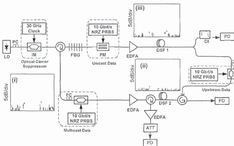
Fig. 3.24 Experimental setup of the modified scheme. Insets show the (i) output spectrum of the PM; (ii) reflected spectrum of FBG; (iii) transmitted spectrum of FBG. Horizontal scale: 0.5nm/div.
