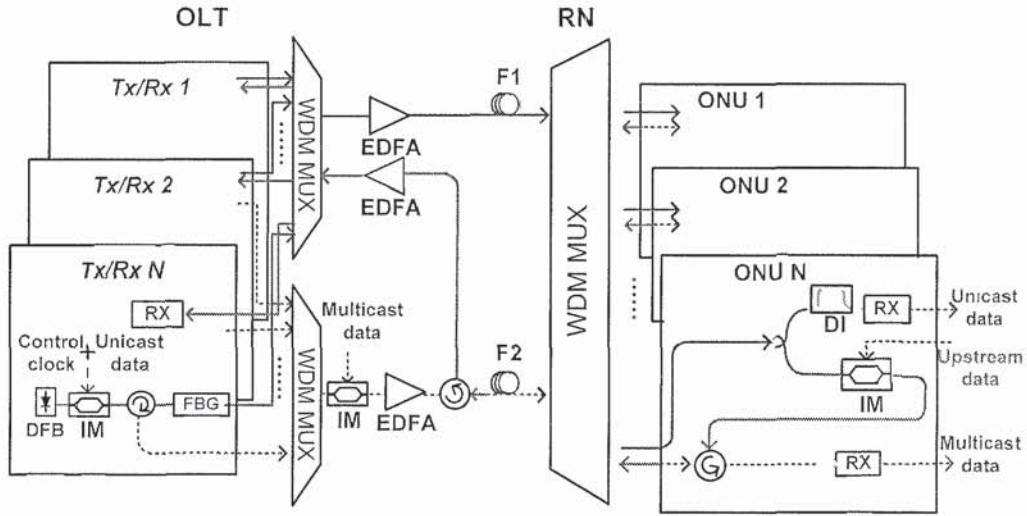
Fig. 3.16 The WDM-PON with OCS optical multicast overlay scheme. F1 & F2: fiber feeders, FBG: fiber Bragg grating, IM: optical intensity modulator, EDFA: Erbium doped fiber amplifier, DI: delay interferometer.
