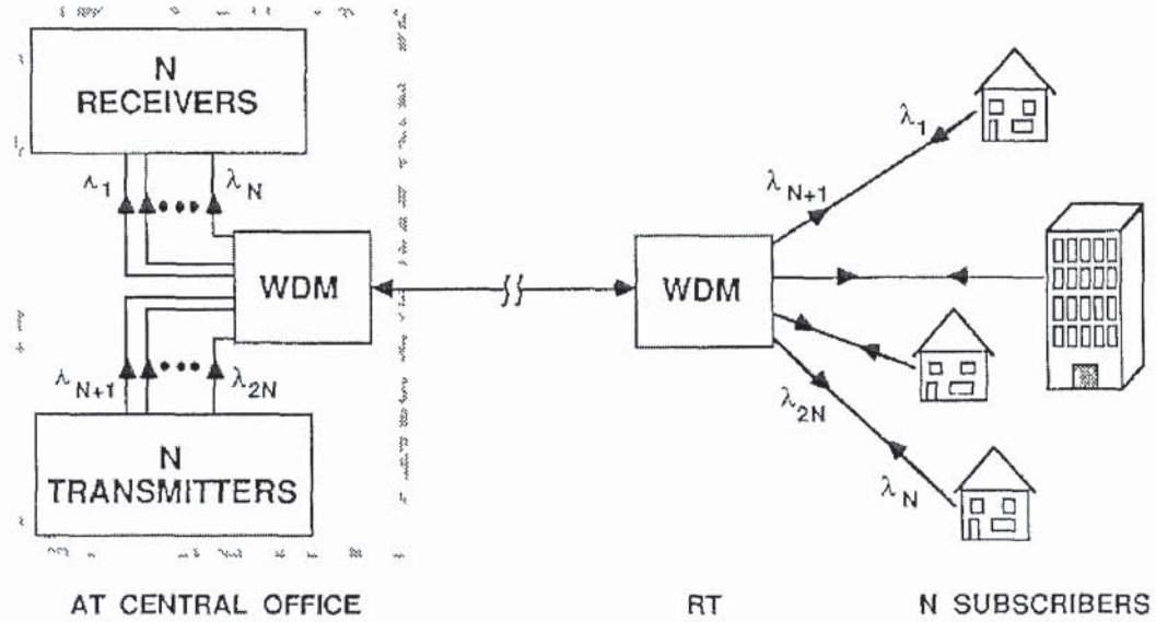
Fig. 2.1 The Passive Photonic Loop architecture providing independent, two-way transmission for N subscribers [21]
