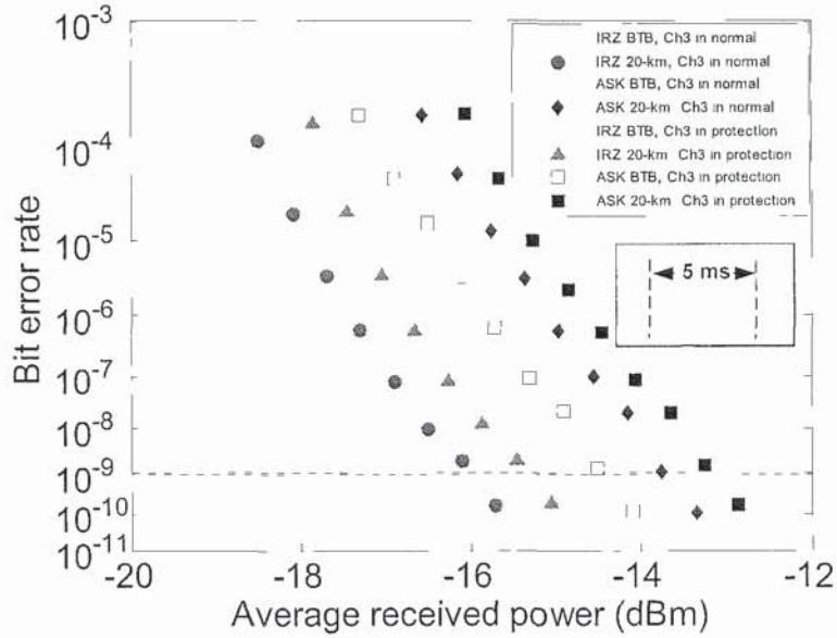
Fig. 4.16 BER measurements for channel 3
