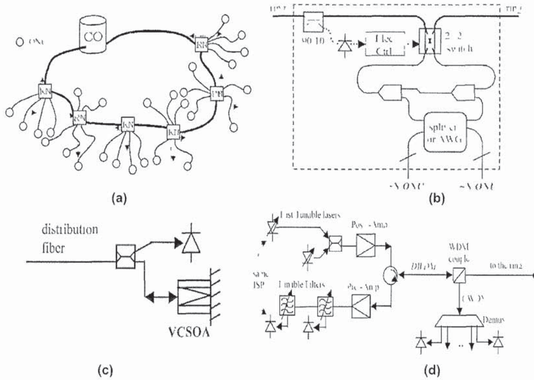
Fig. 2.6 Schematic diagram of SUCCESS [30]. (a) Architecture and topology. (b) Design schematics of remote node with capability of protection and restoration. (c) Design of ONU with Polarization-insensitive VCISOA is used for its better coupling to fiber and higher degree of system integration. (d) Design of transceivers at OLT.
