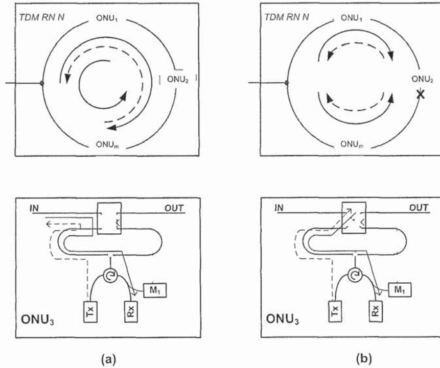
Fig 4 18 TDM RN architecture and the structure of ONU 3 (a) Structures under normal working mode (b) Structures under protection mode in case of a fiber cut between ONU 2 and ONU 3 Solid and dashed arrows show the routing paths of the downstream and upstream traffic of ONU 3 , respectively
