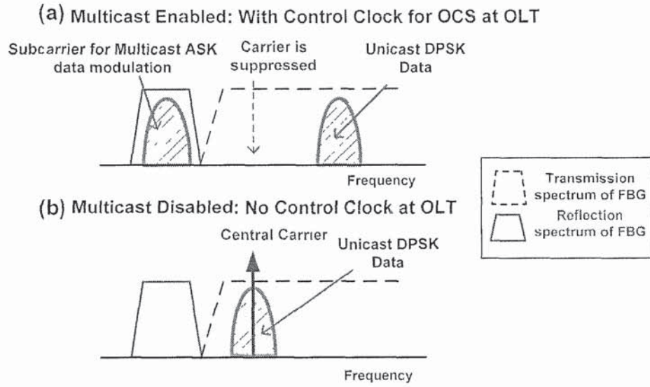
Fig. 3.17 Spectra of downstream carrier to illustrate the principle of multicast overlay control via OCS.
