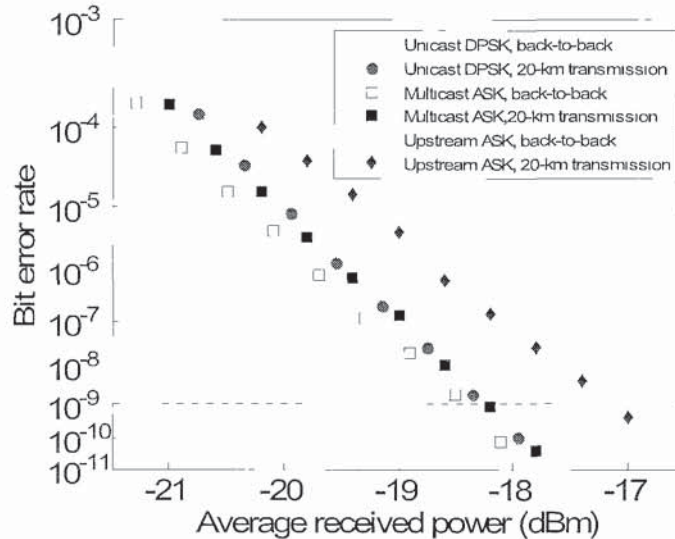
Fig. 3.25 BER measurements when multicast is enabled
