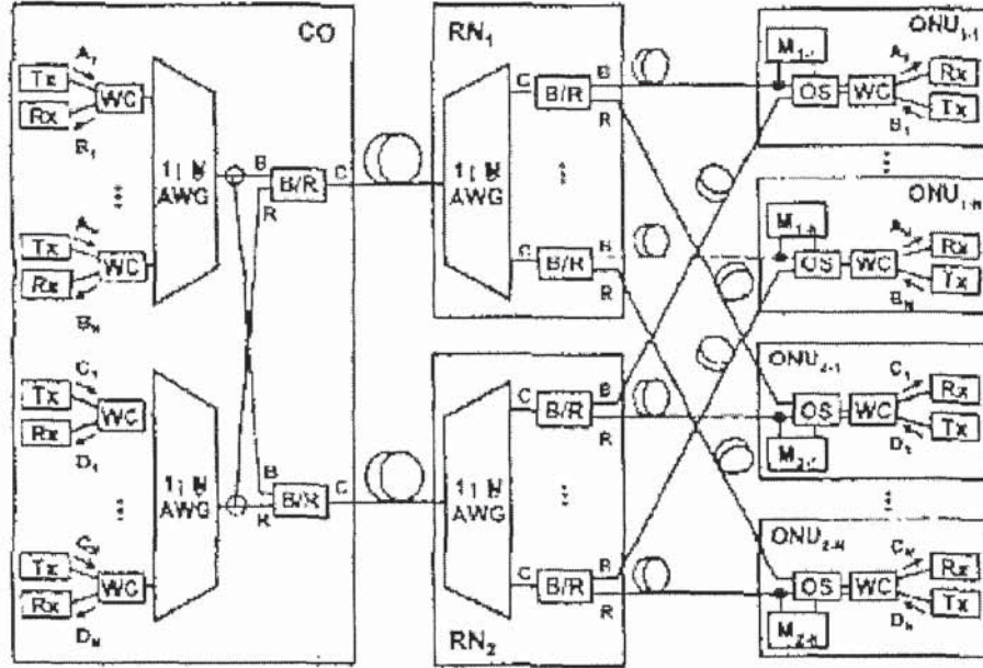
Fig. 4.4 A self-protected survivable WDM-PON in [69]. WC: wavelength coupler, B/R: blue/red filter, OS: optical switch, M: power monitoring unit.
